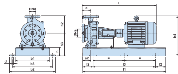
GBS 80-400
